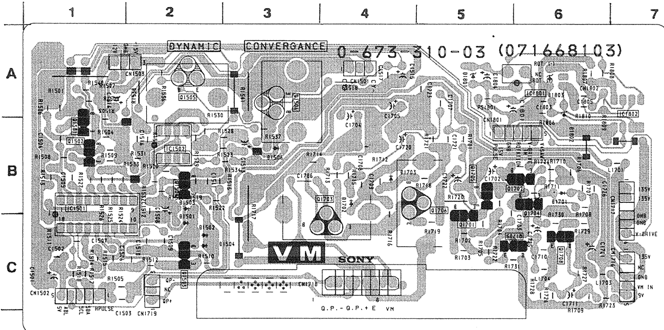
VM Board
