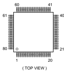
SDA5273M-CP-GEG SDA3OC263-GEG
